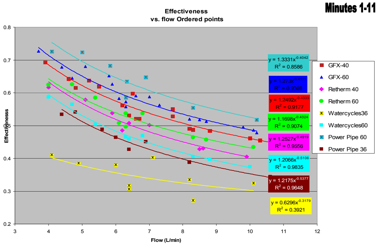
Figure 7: Effectiveness Curves (Minutes 1-11)
