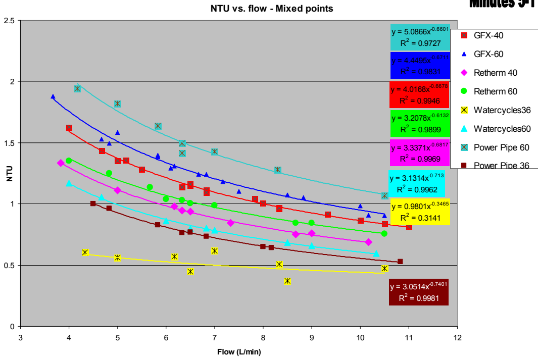
Effectiveness vs. Flow rate curves minutes 1-11
