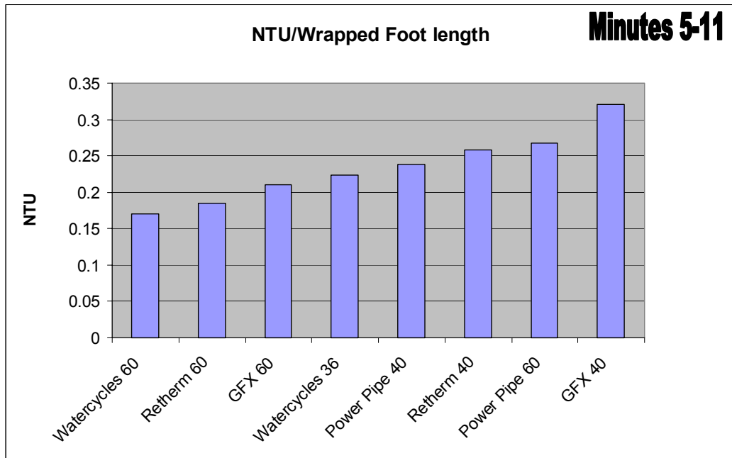
Figure 6: NTU/ Wrapped Foot Length
