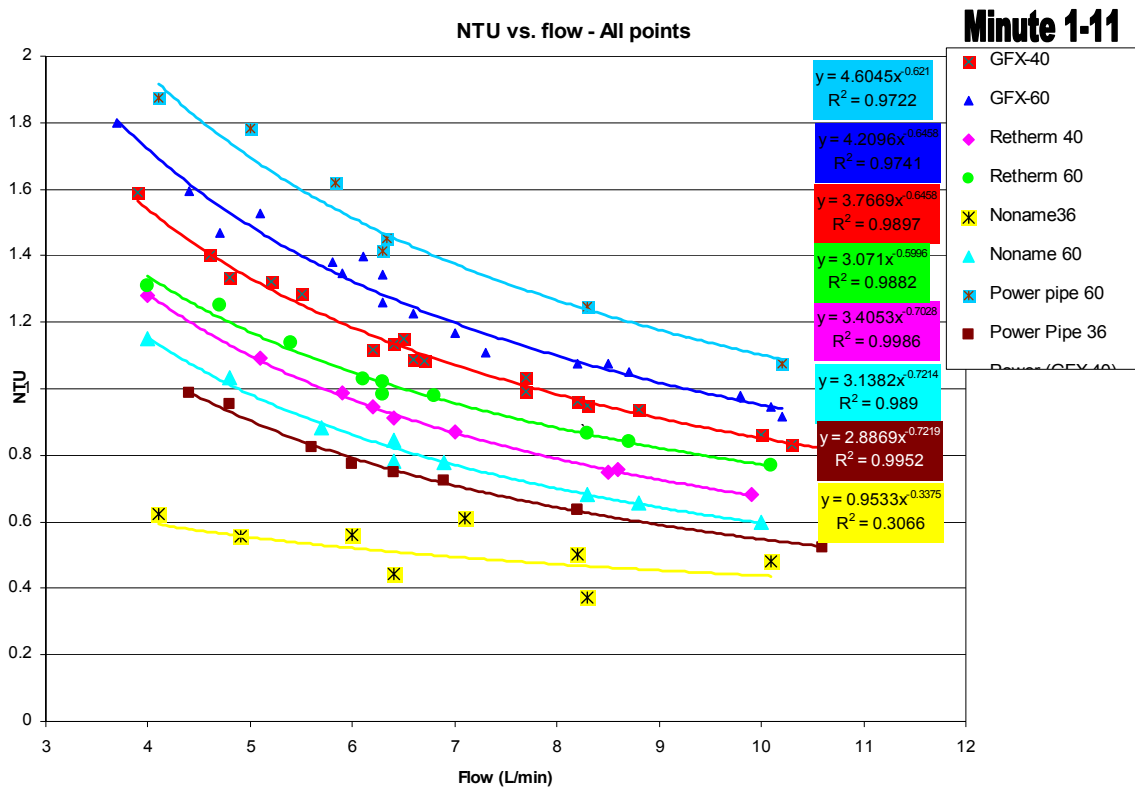
Figure 5: NTU Curves (Minutes 1-11)
