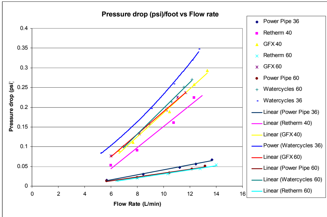
Figure 10: Pressure Drop(psi)/Foot vs. Flow Rate
