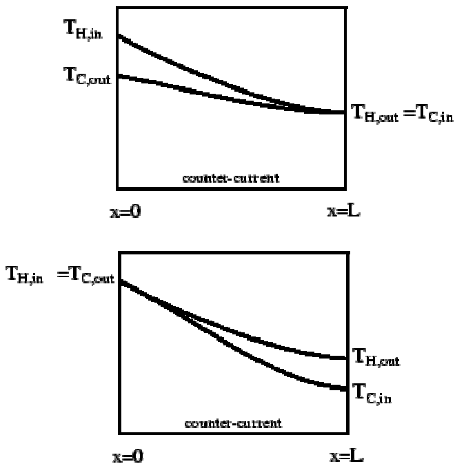
Figure 4: Counterflow HE Temperature Distribution
