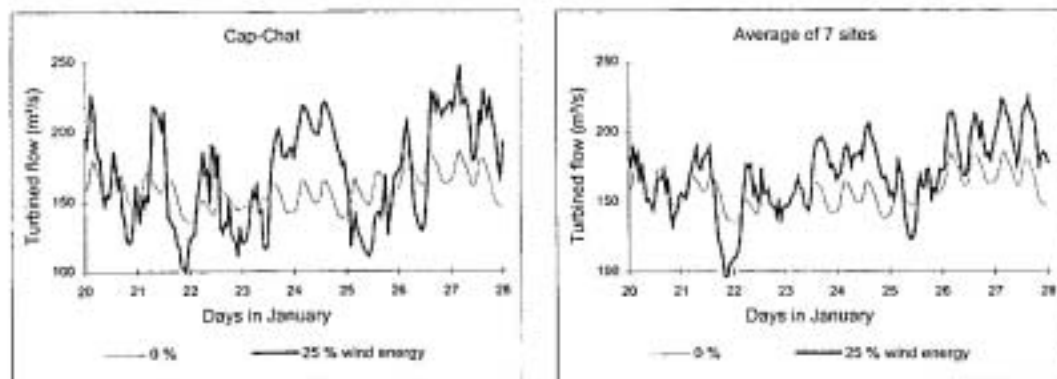
Figure 5. Effect of the Addition of Wind Energy on Turbine Flow
