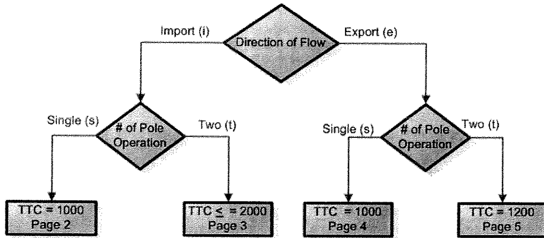
HVDC – TF ATC Process Flow Diagram
