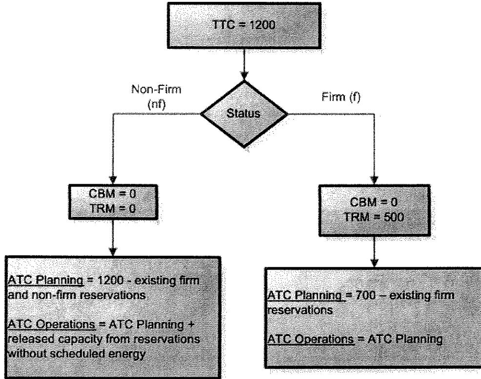
HVDC-TC ATC Process Flow Diagram (export, two-pole operation)
