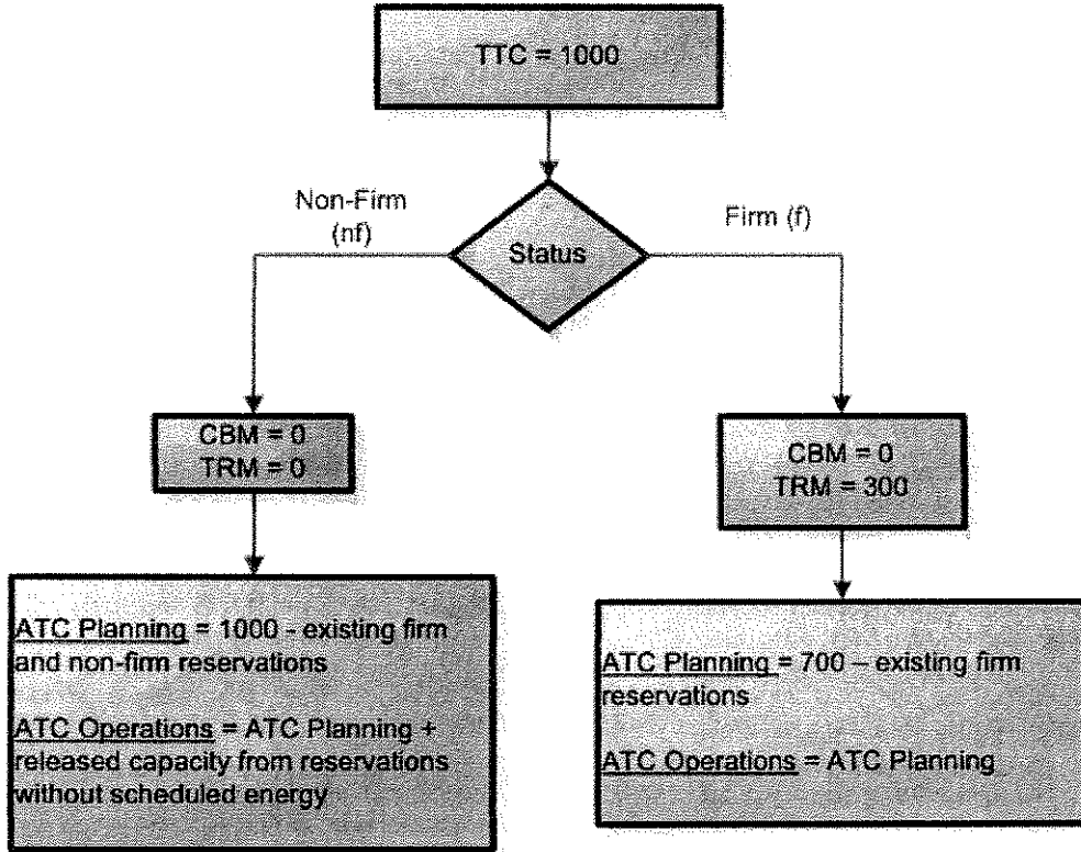
HVDC – TF ATC Process Flow Diagram (export, single-pole operation)
