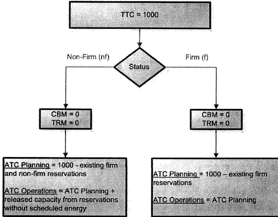
HVDC – TF ATC Process Flow Diagram (import, single-pole operation)
