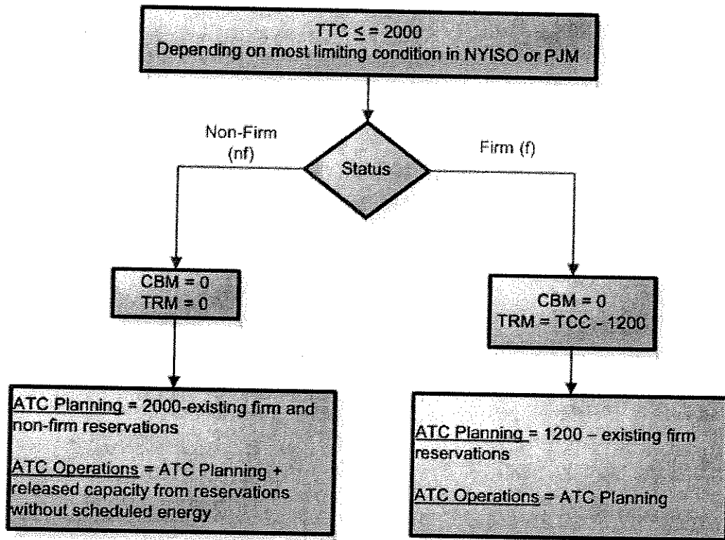
HVDC – TF ATC Process Flow Diagram (import, two-pole operation)
