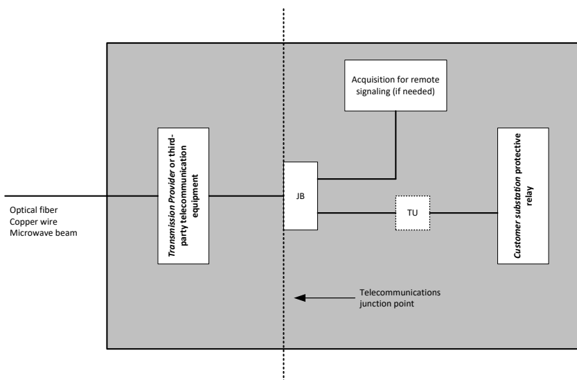
Figure 2 Customer substation telecommunication system
