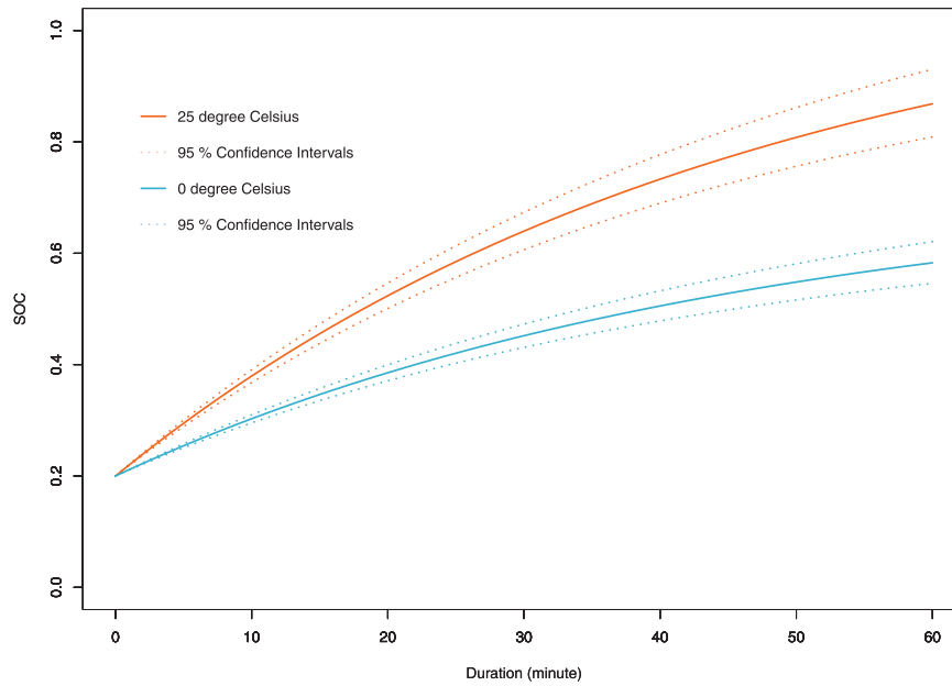
Fig. 4. Plot of predicted SOC profile over time using the smooth approximation function.
