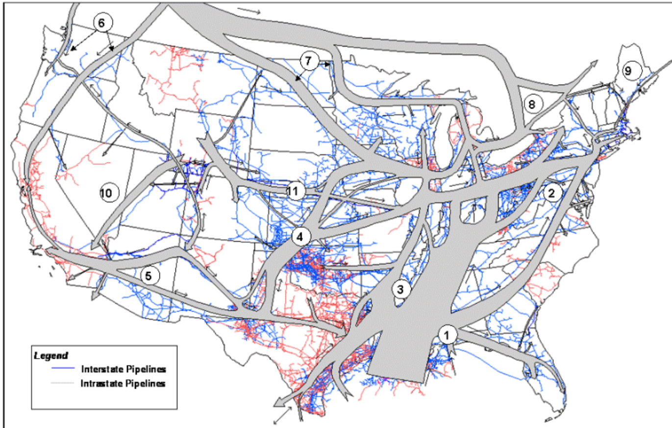
Figure 9. Major U.S. natural gas transportation corridors (2008).
