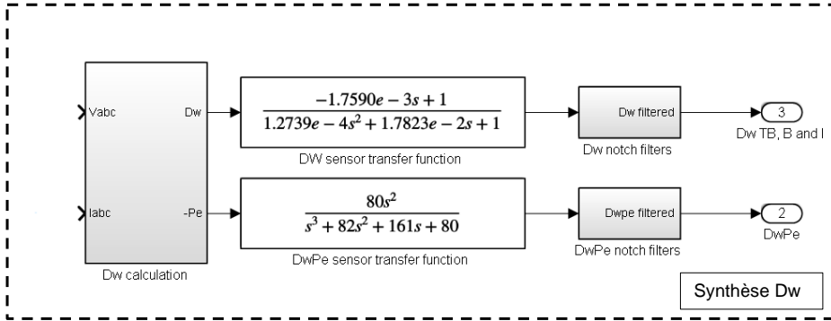
Figure E.2: Rotor Speed synthesis
