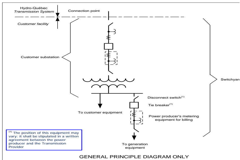
Figure 3: Generating station connected through a customer facility
