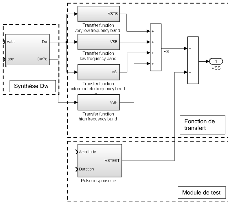
Figure E.1: Simplified scheme of the multiband stabilizer
