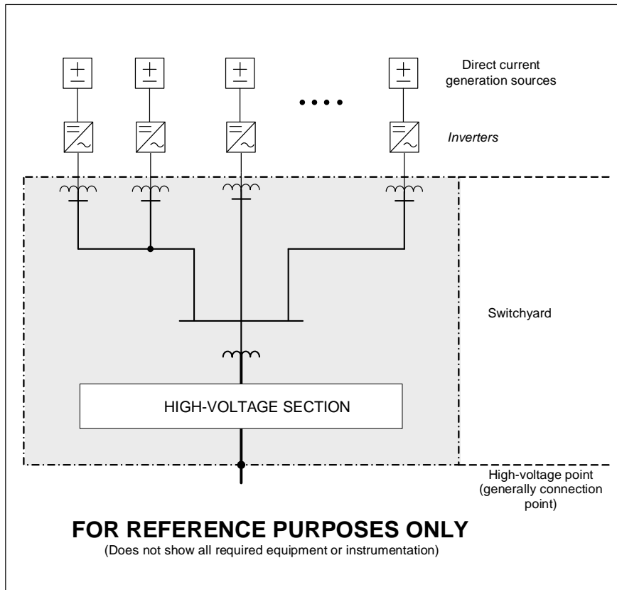
Figure 5: Switchyard for a generating station using SERMOs
