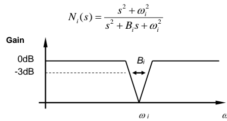
Figure E.3: Notch Filter Characteristics
