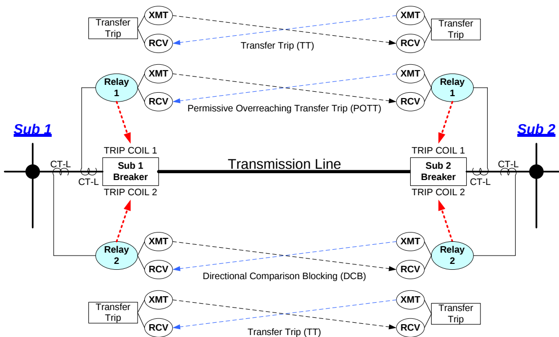
Figure 5–7 — Communication System
