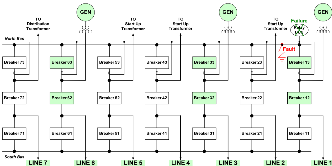
Figure 5–1 — Strong Source System One Line
